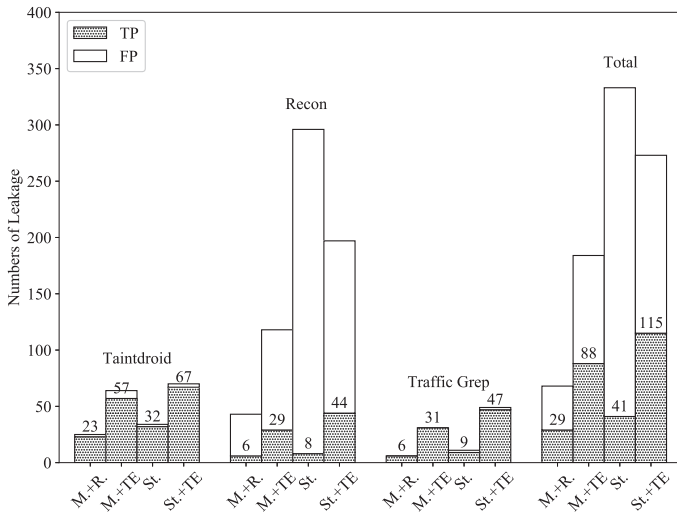
Figure 7. The number of detected privacy leakage of three dynamic analysis, i.e., TaintDroid, ReCon, and a keyword-based traffic search.
